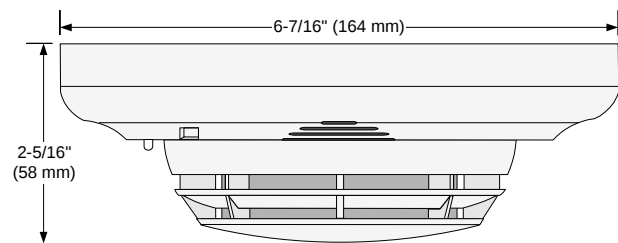
4098-9714 Photoelectric Sensor with Sounder Base
